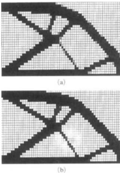
Fig. 7 The optimized result (a) by the conventional approach ( N_{iter}=266 , L=144.1893 , H=0.00394 ) and (b) by the present approach ( N_{iter}=32 , L=143.044 , H=-0.000124 ) (the design domain is discretized by 2048 finite elements.)
