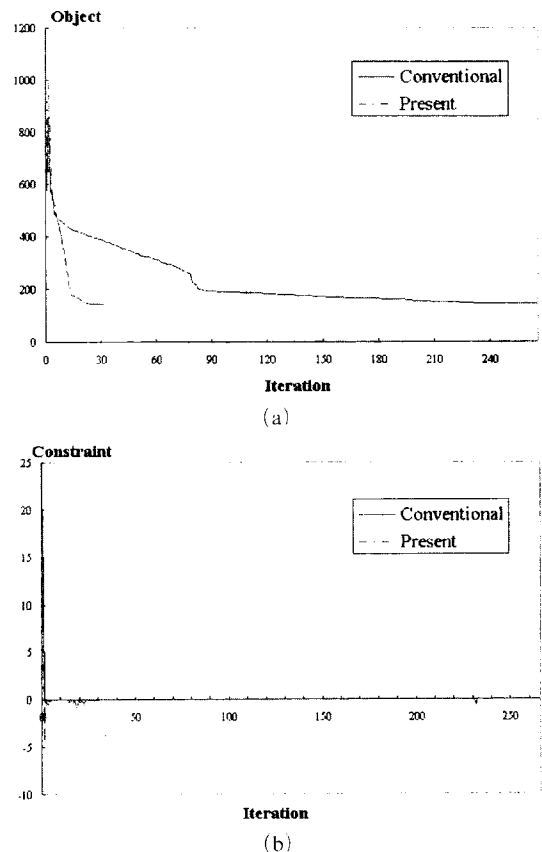
Fig. 8 The iteration histories for the results shown in Fig. 7 : (a) the objective function and (b) the constraint function
