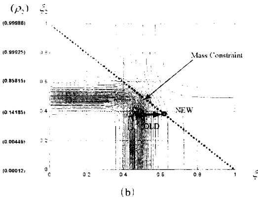
Fig. 3 Old and new design points plotted on the contour plane for (a) L(\rho_1, \rho_2) and (b) \tilde{L}(\xi_1, \xi_2) (the design variables used for (a) and (b) are (\rho_1, \rho_2) and (\xi_1, \xi_2) , respectively)
