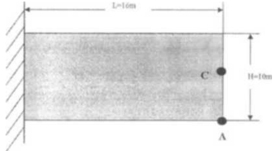
Fig. 5 Design domain with one side clamped ( L=16\text{ m} , H=10\text{ m} , E=200 \times 10^5\text{ Pa} , \nu=0.3 , mass constraint=37.5% (60/160))
