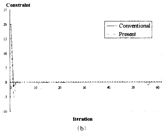
Fig. 10 The iteration histories for the results shown in Fig. 9: (a) the objective function and (b) the constraint function
