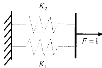
Fig. 2 A model system consisting of a rigid block and two elastic springs
